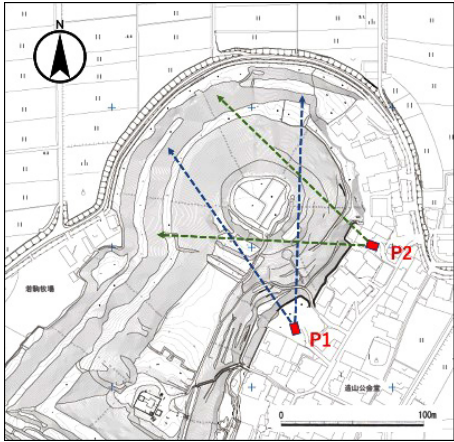
Fig. 2 Locations and range of measurement. Two positions, designated P1 and P2, were selected for muographic measurements, with the instrument oriented towards the posterior circular mound. The measurement range of the instrument was 1000 mrad (57.3 degrees). A contour map of the burial mound, used with permission from the Okayama City Board of Education (2014).
