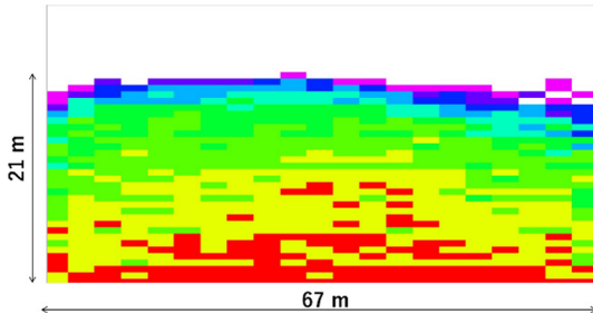
Fig. 4 Measurement result of muon transmission image at location P1. The measurement period was 93 days. The figure shows distribution of muon count numbers reached the detector through the mound. To decrease influence of noise, five pixels were binned in the horizontal direction, therefore, one pixel corresponds to 39.1 \times 7.8 mrad in visual angle. The intensity of pixels were obtained as a gray scale image (normalized between 0 to 1) and they were colored in hue order 0 to 360 degrees.
